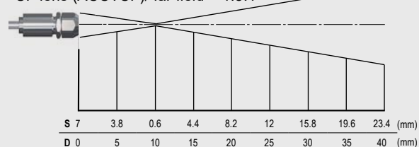
Optics CTi LT SF, D:S = 22:1, with additional CF lens (ACCTCF)/ far field = 1.5:1
